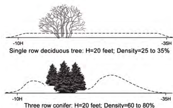
FIGURE 3 Effect of shelterbelt density on snow accumulation
