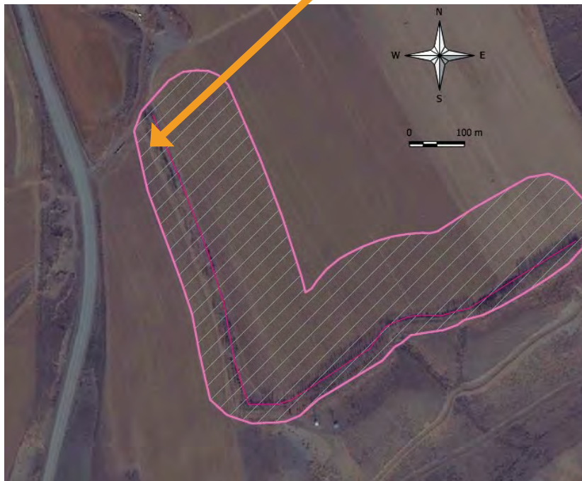
The planted shelterbelt from above, and an estimate of the quiet area created by protection from winds from the west and south (area estimate = 10 \times height on the leeward side, and 3 \times height on the windward side; windbreak is the dark pink line and the quiet area is in light pink). The shelterbelt is approximately 15 metres high, and is about 1.2 km in length.
