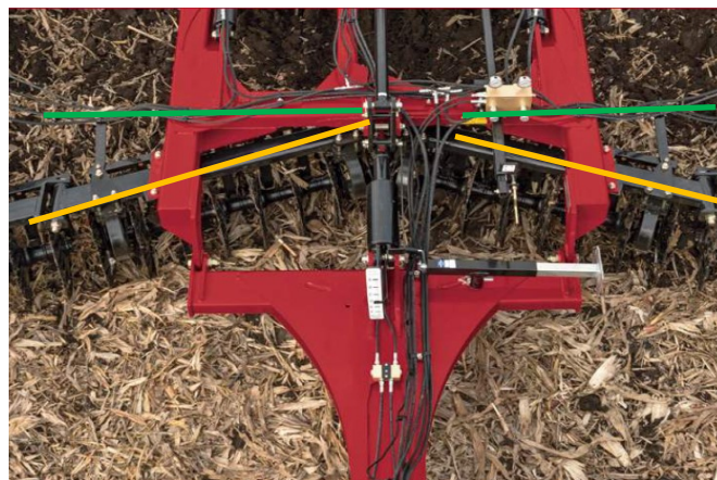
A Horsch high speed tillage disc working up perennial forage stand in the fall after being sprayed out.
