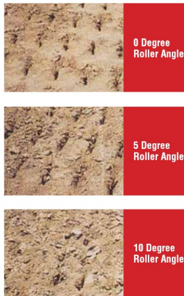
Figure 3: Illustrating the angle changes and the resulting soil disturbance on the right. This tool has been useful in increasing water infiltration in coarse textured soils in the Peace.
